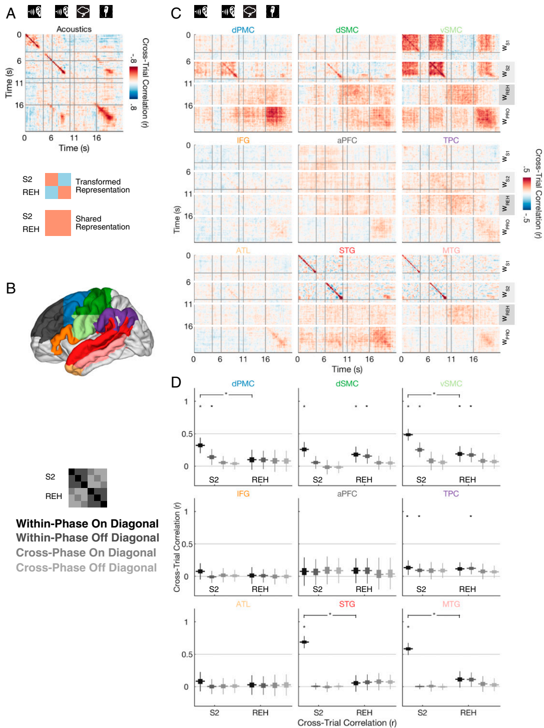
Fig. 4. Temporal specificity of sentence-locked activity. (A) Cross-time, cross-trial correlation maps for the amplitude of the recorded acoustics. A positive correlation at time (t_1, t_2) indicates that higher amplitude values at time t_1 on the first presentation of a sentence were associated with higher amplitude values at time t_2 on the second presentation of the sentence. Thus, a positive correlation along the diagonal ( t_1 = t_2 ) indicates that amplitudes are not only sentence specific but also locked to individual time points within a stimulus. Correlation values are averaged across coherent and incoherent sentences. The vertical gray lines indicate the onsets of the silent gap following S1 and S2, silent gap following S2, and the silent rehearsal cue, respectively. (B) Schematic of color-coded ROIs. (C) Cross-time, cross-trial correlation maps of the neural data within each ROI (similar to A, but with correlations computed for weighted cortical broadband power timecourses). All correlations along one row of the time–time correlation matrix are computed using the region-specific weights derived from a single phase (e.g., perception, rehearsal, or production phase). W_{S1} , weights from the S1 perception phase; W_{S2} , weights from the S2 perception phase; W_{REH} , weights from the rehearsal phase; W_{PRO} , weights from the production phase. (D) Statistical summary of the cross-time, cross-trial correlation values shown in A ( q < 0.05 , FDR corrected across ROIs and number of comparisons within phase). The distribution of correlation values is shown for the within-phase on-diagonal component ( t_1 = t_2 , black), the within-phase off-diagonal component (dark gray), the cross-phase on-diagonal component (lighter gray), and the cross-phase off-diagonal component (lightest gray) of the correlation matrix. Results are summarized separately for the S2 phase and the REH phase for each ROI. The thicker horizontal line represents the median of the out-of-sample correlation distribution, while the box width represents its interquartile range. The vertical thin lines extend to the minimum/maximum of the out-of-sample correlation distribution, excluding outliers.
